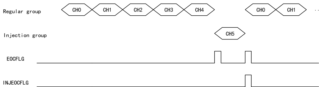
Figure 108 Automatic Injection Timing Diagram
