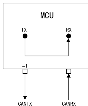
Figure 98 CAN Works in Silent Loopback Mode
