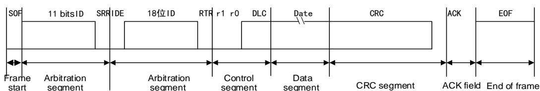
Figure 95 Extended Data Frame
