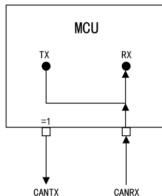
Figure 96 CAN Works in Silent Mode
