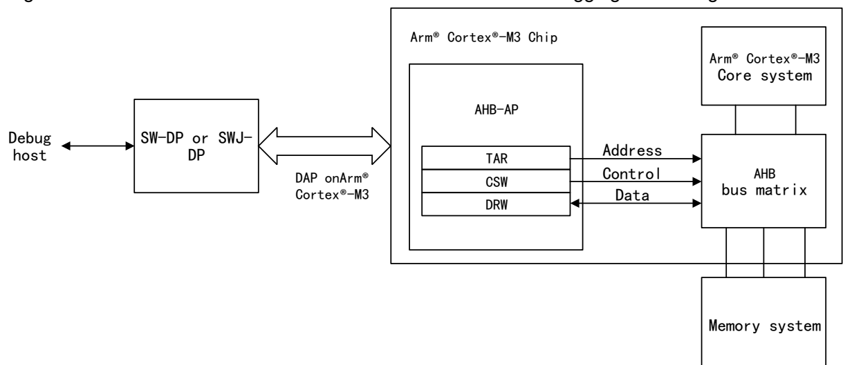
Figure 15 APM32A10xxx Level and Arm® Cortex® -M3 Level Debugging Block Diagram
